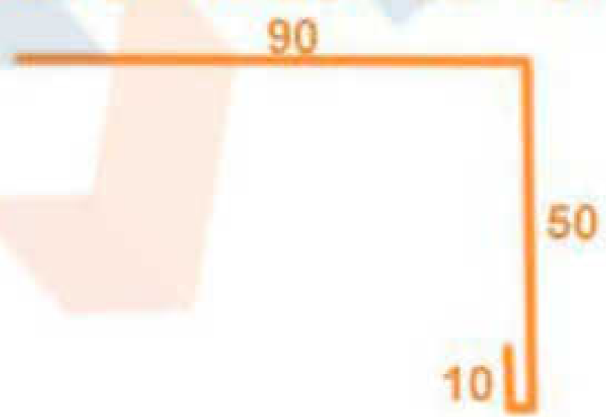
TRIM UNDER WINDOW
