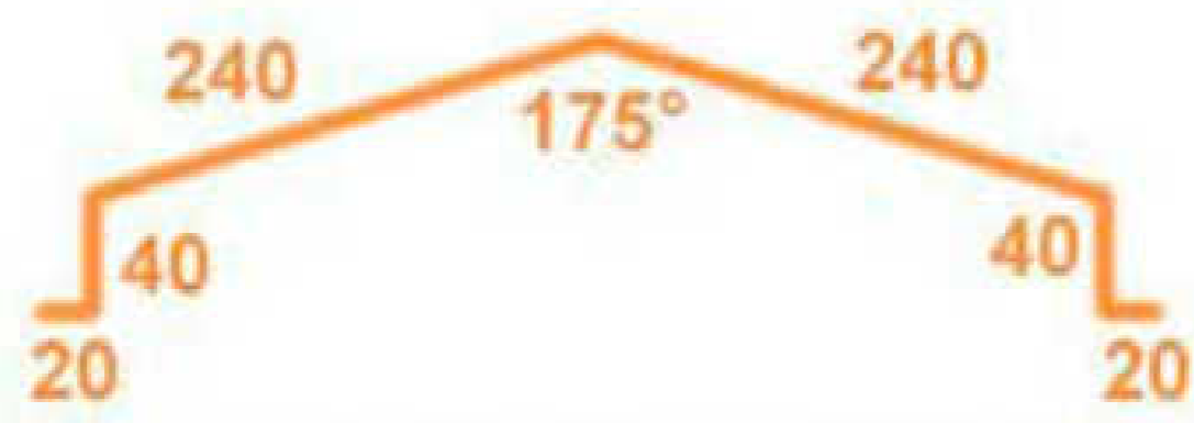
EXTERNAL RIDGE CAPPING
