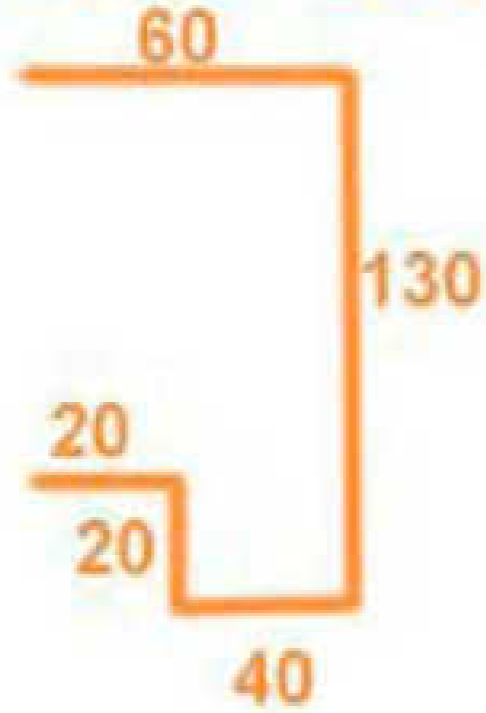
EAVE TRIM
