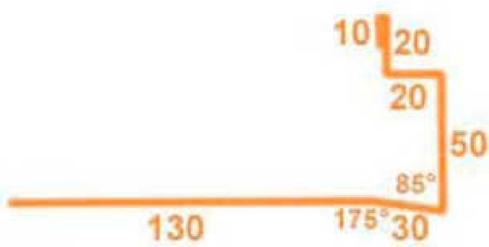
TRIM FOR WINDOW HEAD
