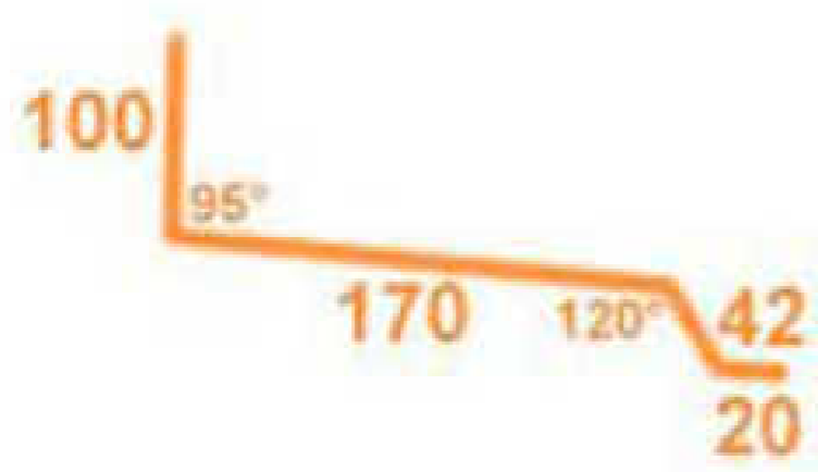
GABLE FLASHING
